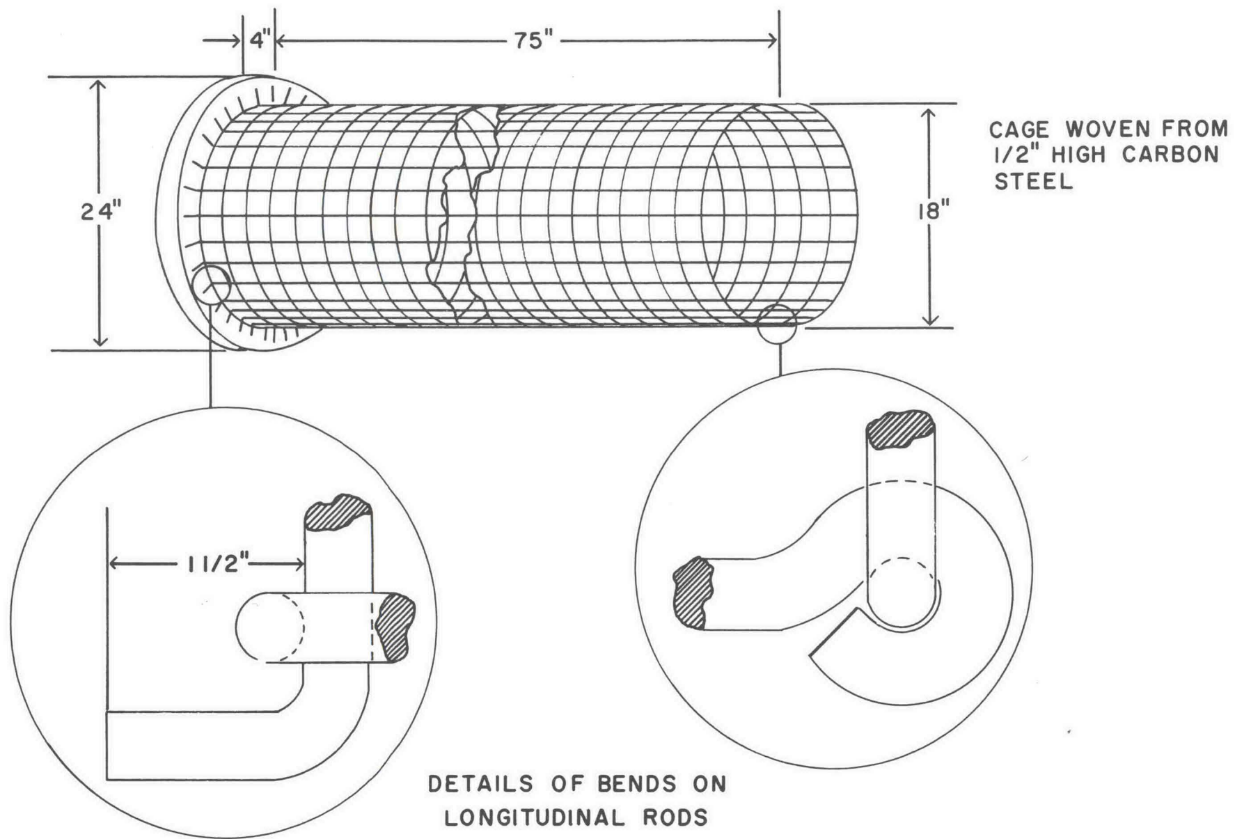
Fig. 10. Wire cage for stopping projectile. In operation the cage is stuffed with rags.
